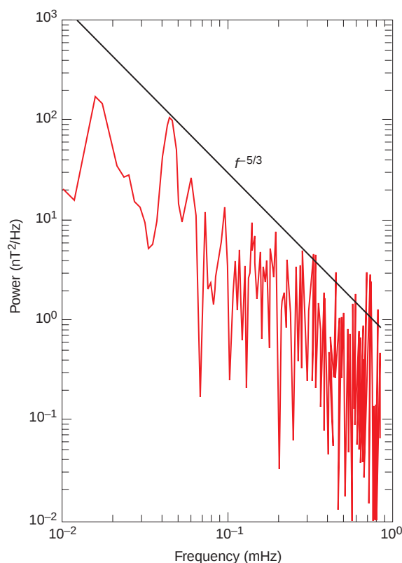
Figure 3. Power spectrum of 10-min data from the x -axis sensor of the Magnetic Field Instrument for the 6-day period, 18–23 June 1996. The higher frequency part of the spectrum shows a frequency dependence of f^{-(5/3)} , which is the representative spectrum for turbulence, and which is typically found for magnetic field fluctuations in the solar wind.
