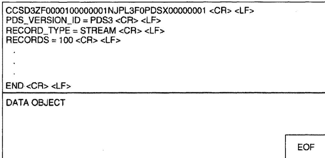
Figure 16.3: SFDU Example
