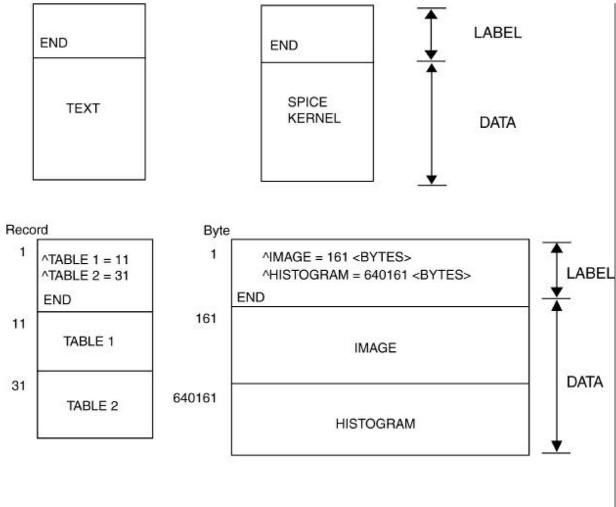
Figure 5.5 Data Object Pointers-Attached Labels
