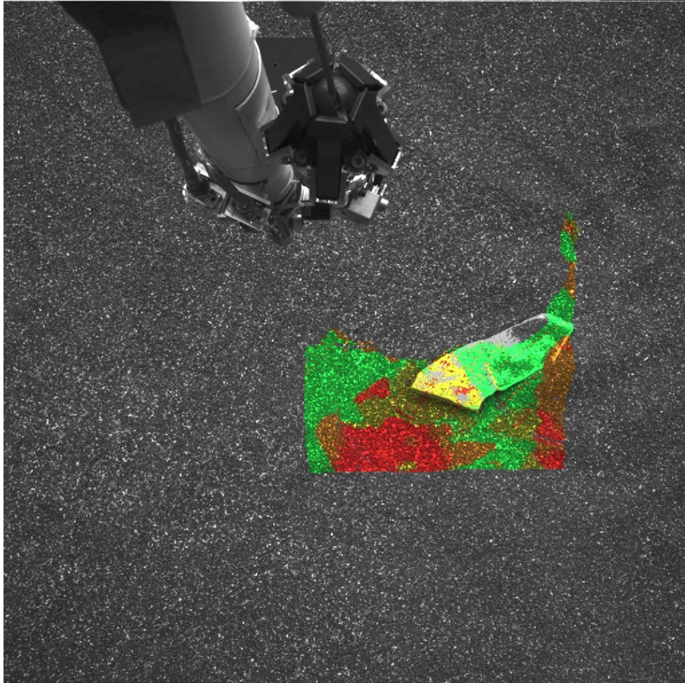
Figure 5-14: Goodness for HP3 (GUH) Data Overlaid onto Image EDR
