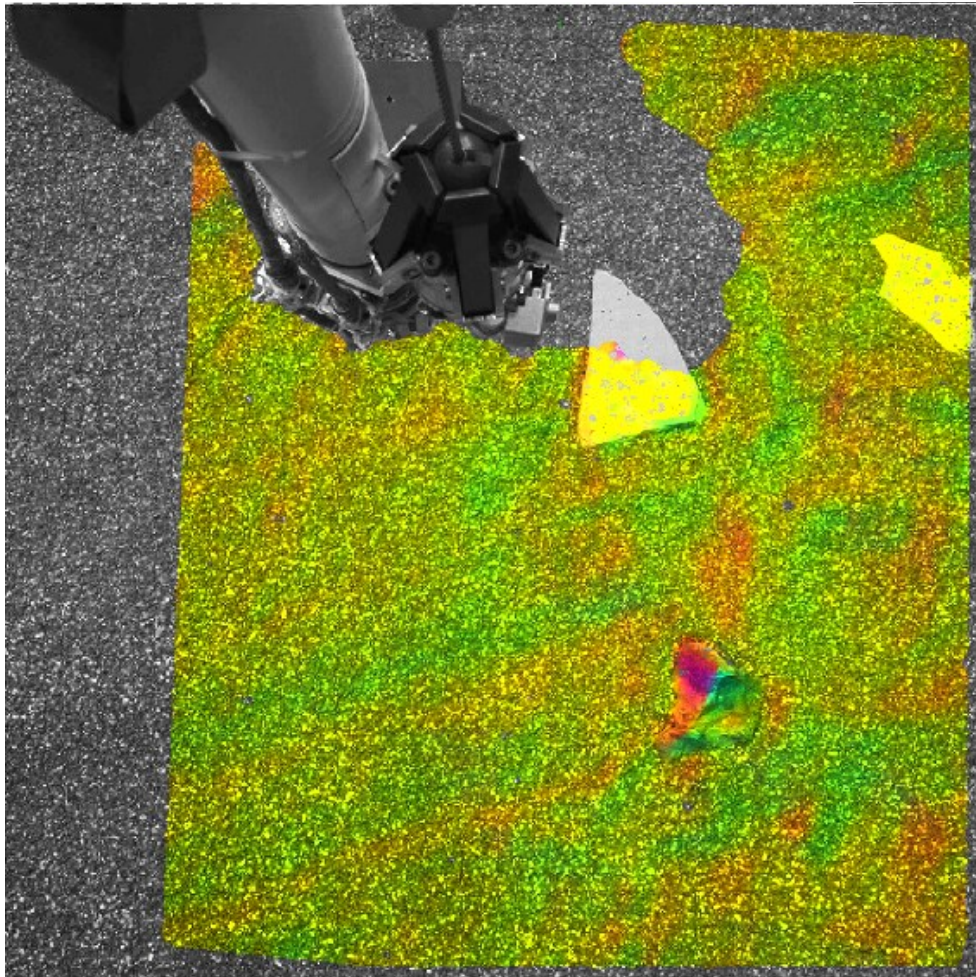
Figure 5-6: Surface Normal Data Overlayed onto Image EDR. RGB colors map directly to XYZ components of the surface normal
