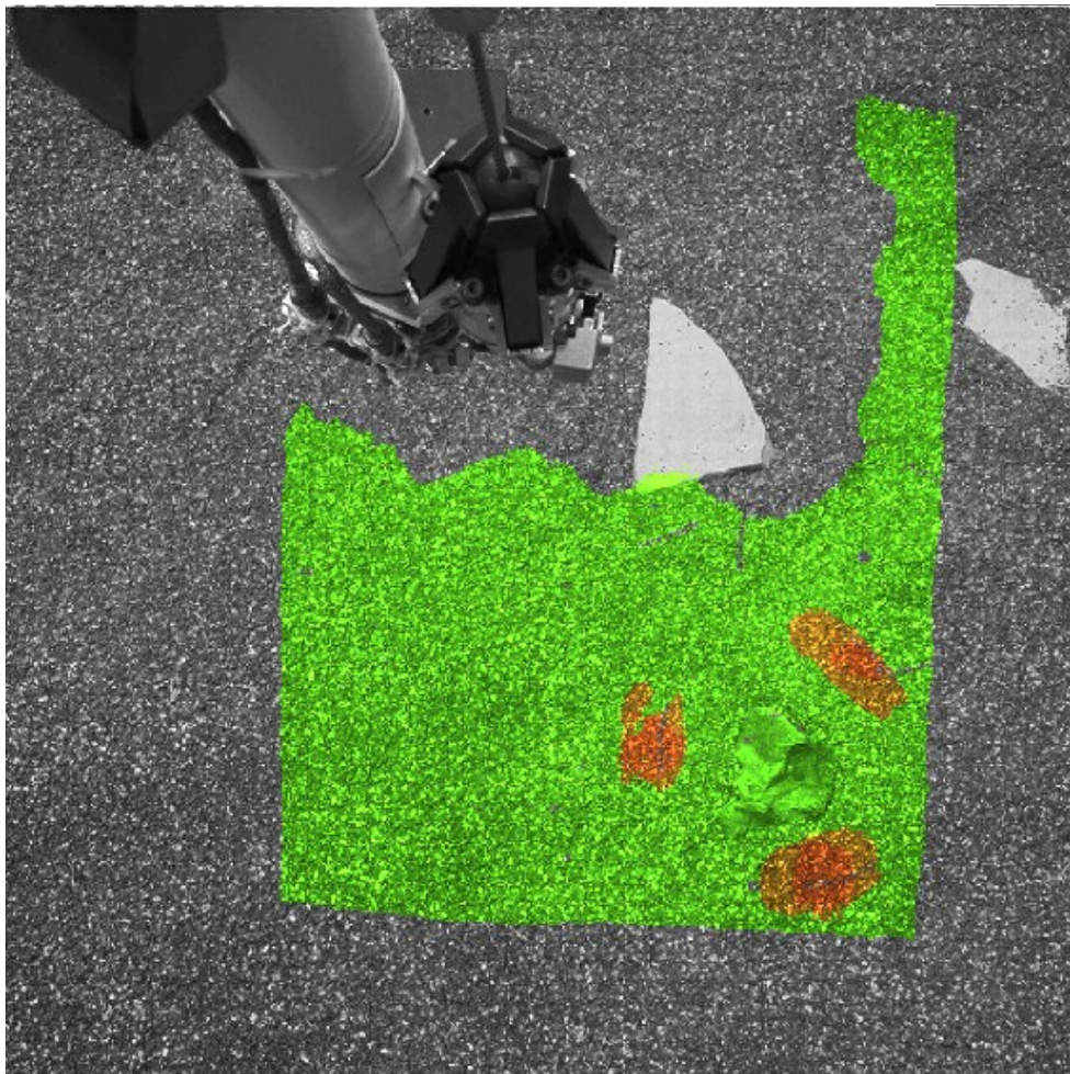
Figure 5-13: Instrument Roughness for SEIS (RUS) Data Overlaid onto Image EDR
