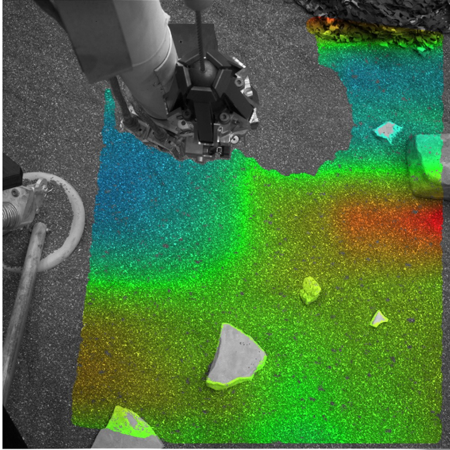
Figure 5-8: Slope Radial Direction (SRD). Data ranges from -7 degrees (blue) to +8 degrees (red)
