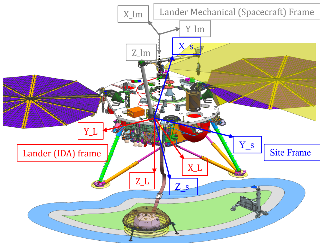
Figure 6-1: InSight Coordinate Systems. Red captions show axes for Lander frame, blue for Site frame, and gray for Lander Mechanical.
