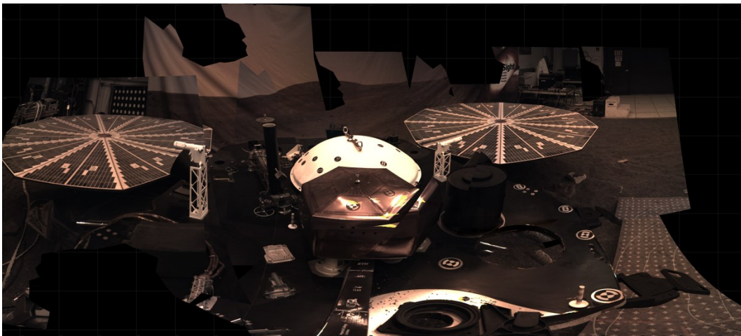
Figure 2-3: Lander horizontal IDC mosaic
