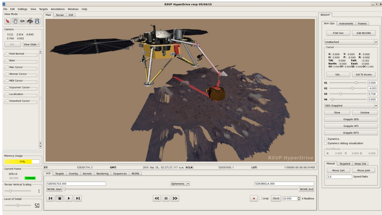
Figure 5-16: Instrument Deployment Location Rendered in Unified Terrain Mesh
