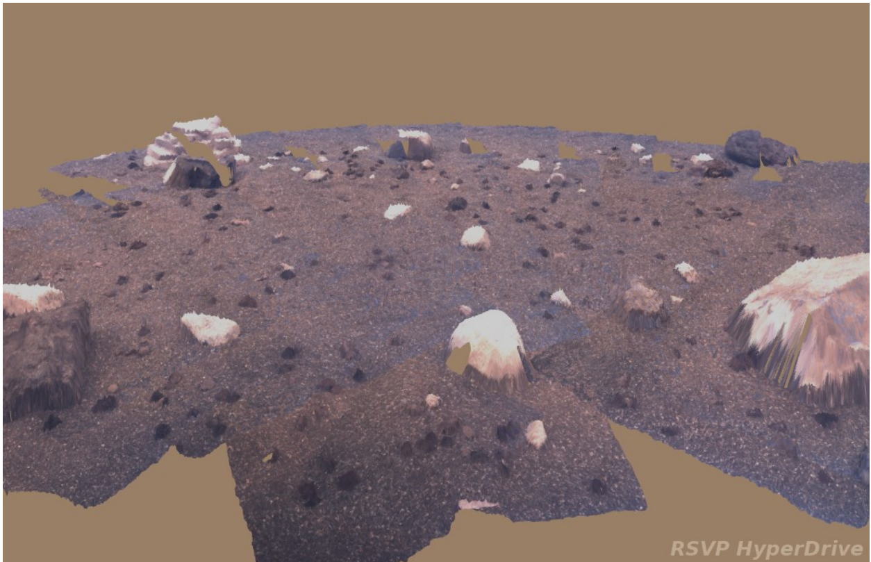
Figure 5-15: DeploymentWorkspace Rendered in Unified Terrain Mesh
