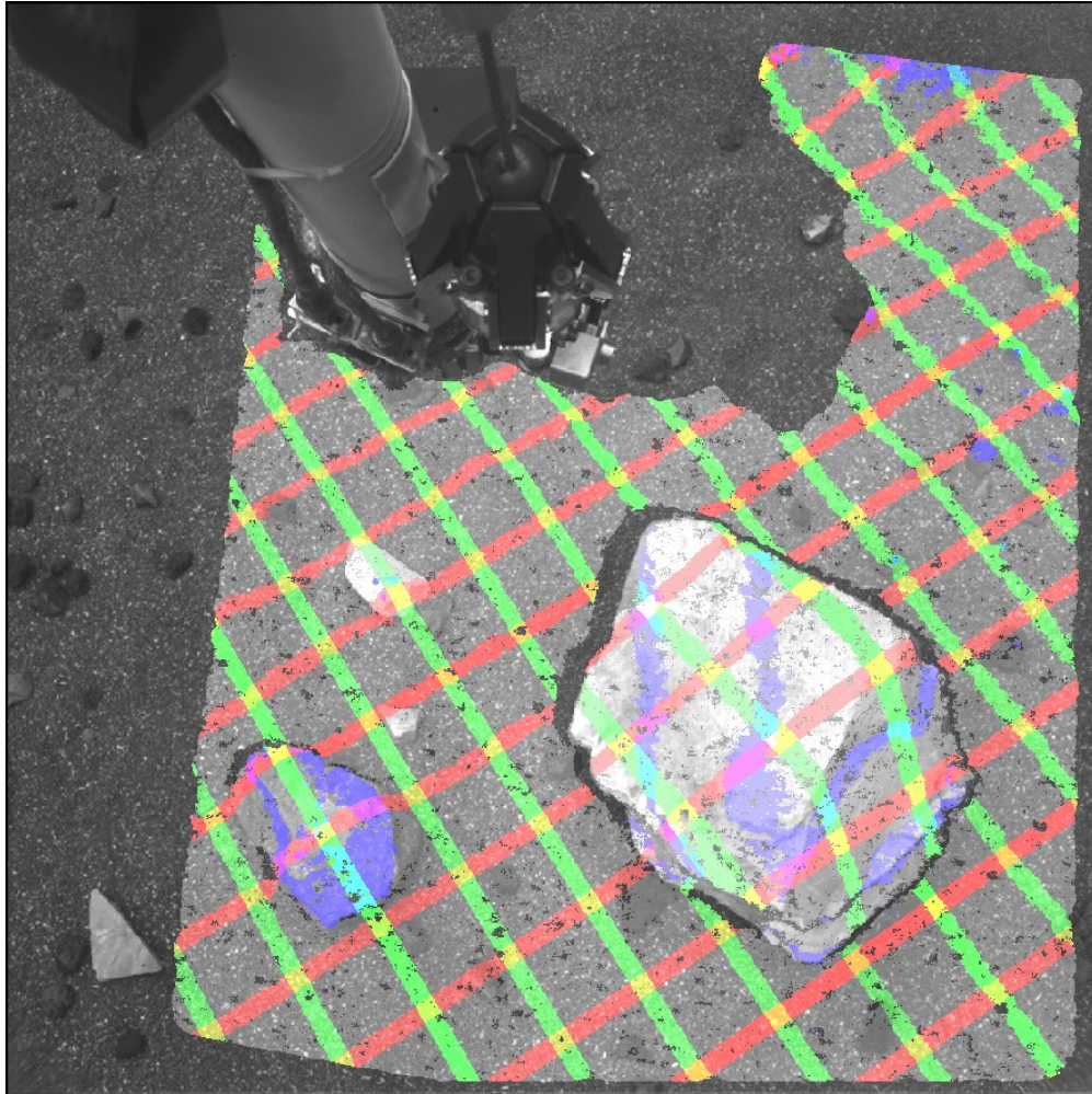
Figure 5-4: XYZ Data Masked and Overlaid onto Image EDR. Red, green, blue indicate lines of constant X, Y, Z respectively at 0.1m spacing (blue lines are thus traditional elevation contours).
