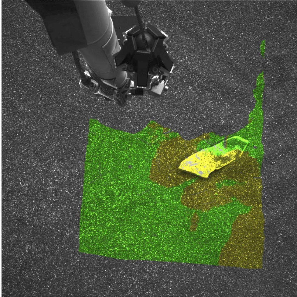
Figure 5-11: Instrument Tilt for SEIS (TFS) Data Overlaid onto Image EDR
