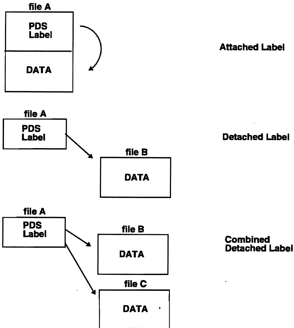
Figure 5.1 Attached, Detached, and Combined Detached PDS Labels
