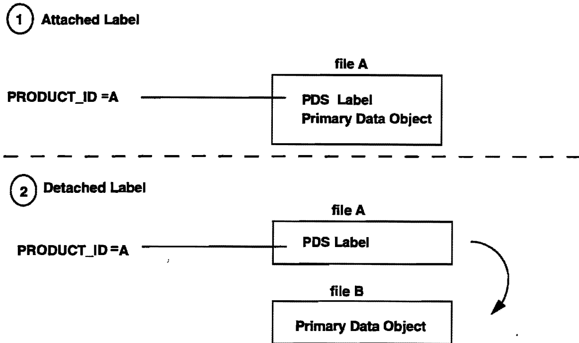
Figure 4.1 Data Product with a Single Data Object
