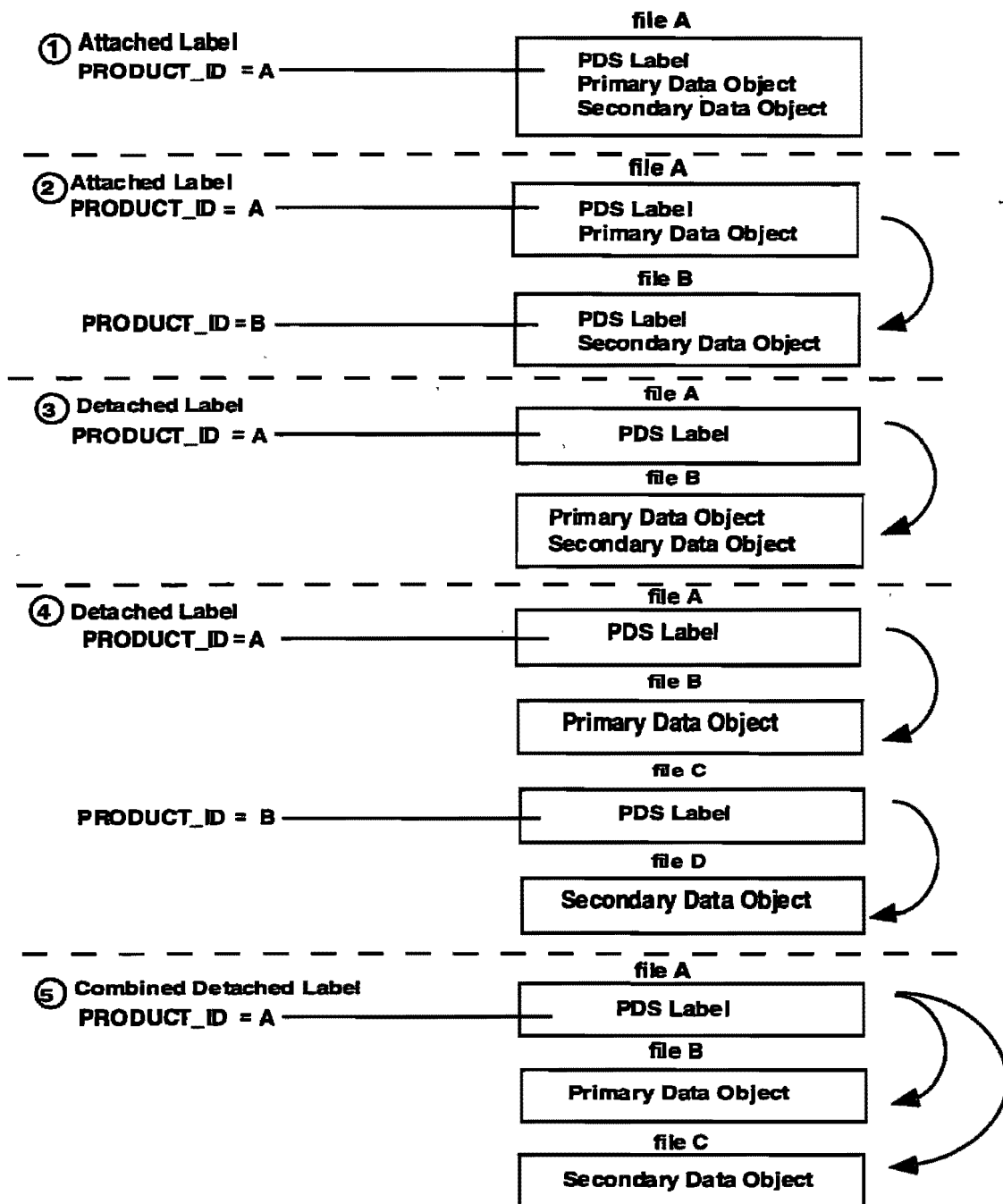
Figure 4.2 Data Product with Multiple Data Objects
