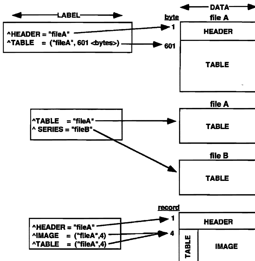
Figure 5.6 Data Object Pointers-Detached & Combined Labels
