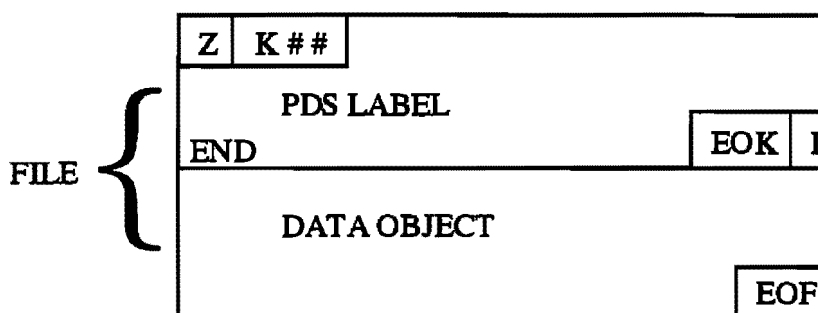
Figure 16.4: PDS Label Example for AMMOS compatible products
