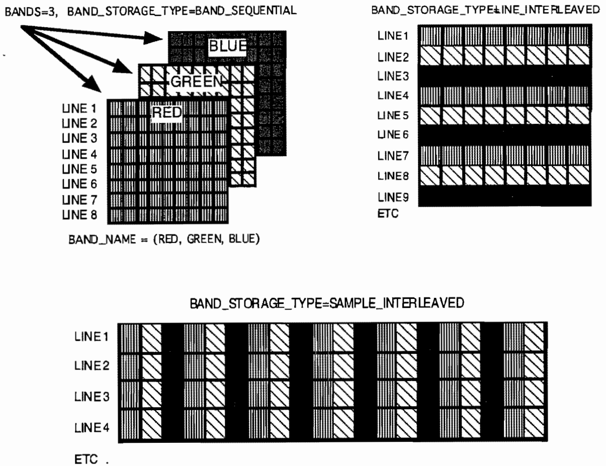
Figure A.2: Keywords for a Multi-Band Image
