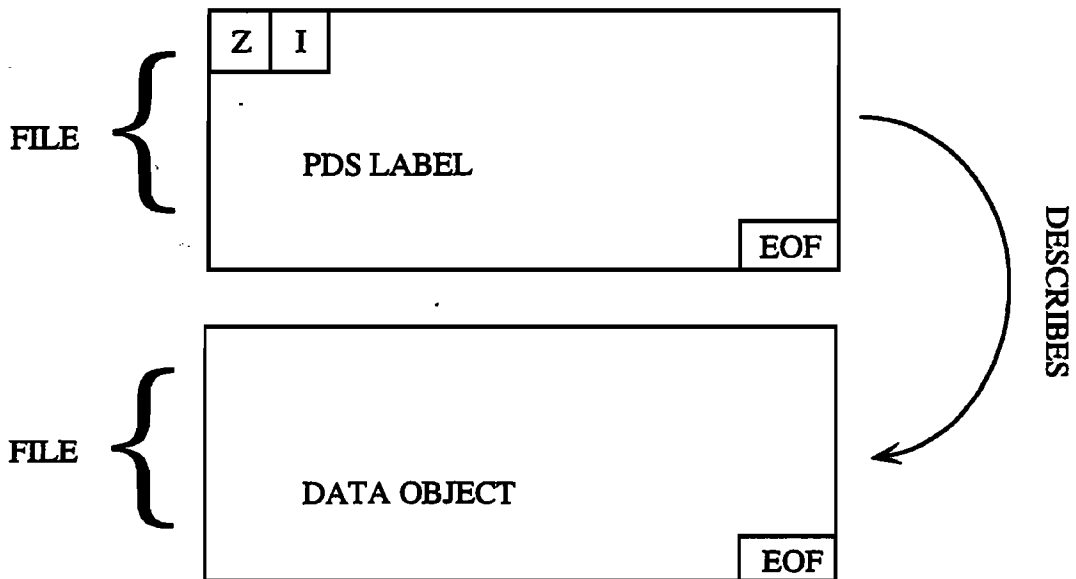
Figure 16.2: Detached PDS Label Example for non-AMMOS compatible products
